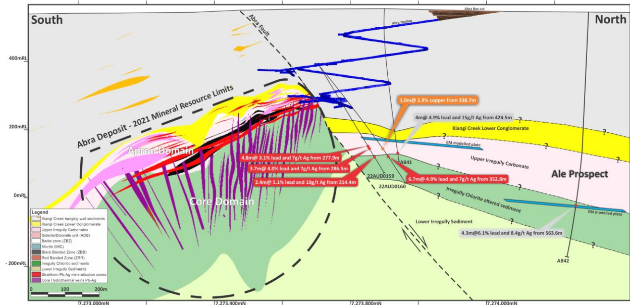
Figure 2. Cross-section looking West of the Abra Deposit and the drilling intercepts from the underground drill holes 22AUD0159 and 0160, as well as the historical drill holes AB41 and AB42, north of the Abra Fault, along with the electromagnetic modelled plates. Current 2021 Abra Deposit Mineral Resource limits is outlined by the thick dashed black line.
