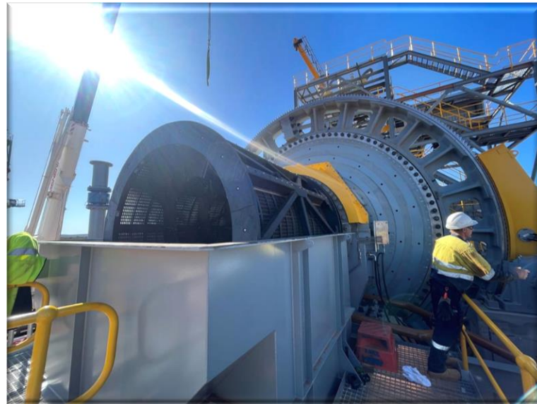
Mill Discharge Assembly
