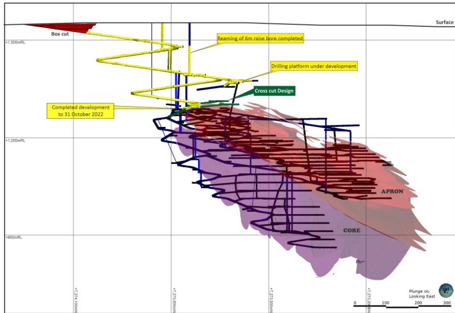
Abra Mine Schematic (October 2022)
